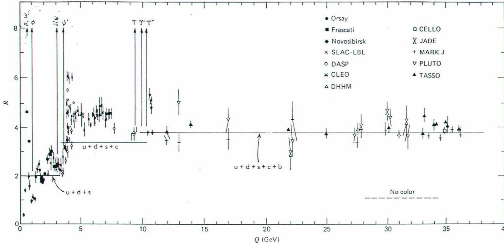
Fig. 11.3 Ratio R of (11.6) as a function of the total e^-e^+ center-of-mass energy. (The sharp peaks correspond to the production of u, d, s, c, b resonances just below or near the flavor thresholds.)
